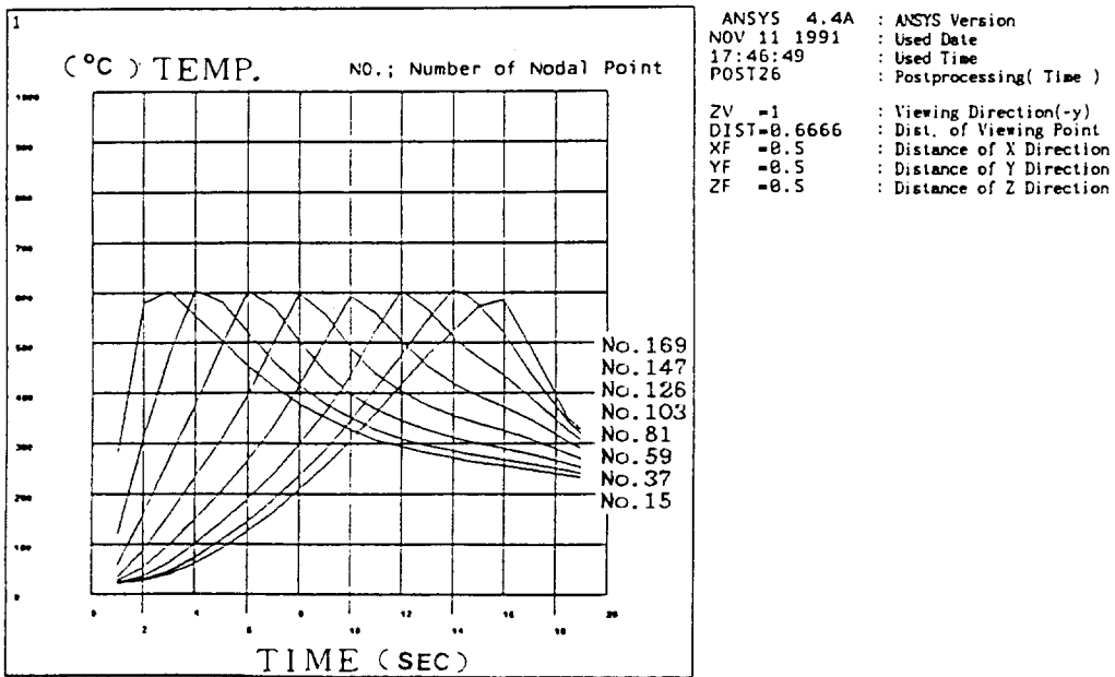
Fig. 12 Temp. vs. Time by Optimal Heat Input(Al-alloy)
