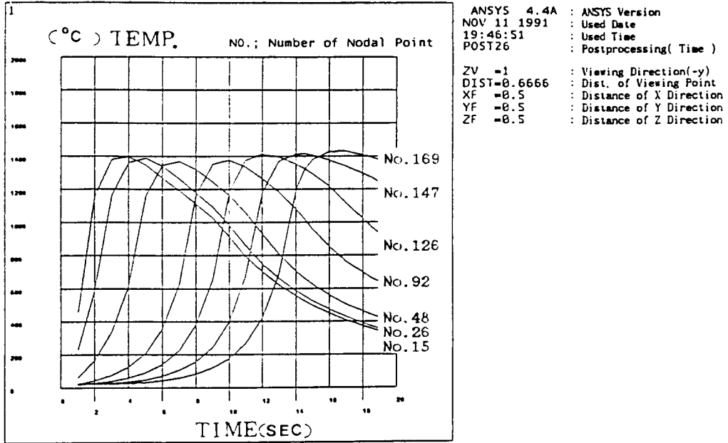
Fig. 11 Temp. vs. Time by Optimal Heat Input(Mild Steel)
