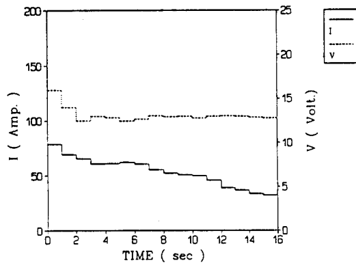
Fig. 8 Current and Voltage by Optimal Heat Input(Al-alloy)
