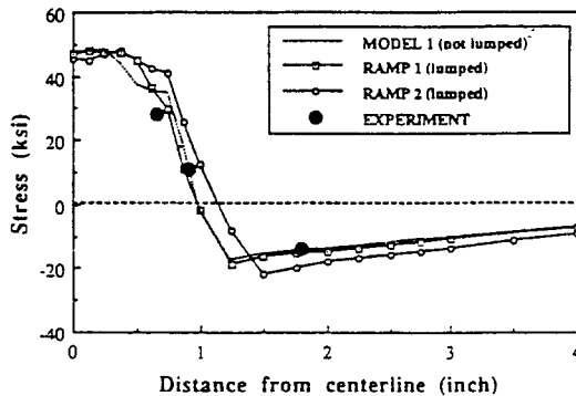
Fig. 15 Longitudinal residual stress distribution at the top surface of the 1-inch thick plate with double-V groove
