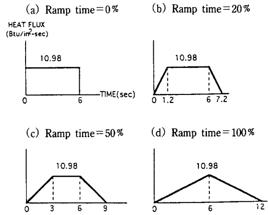
Fig. 5 Ramp functions for different ramp times
