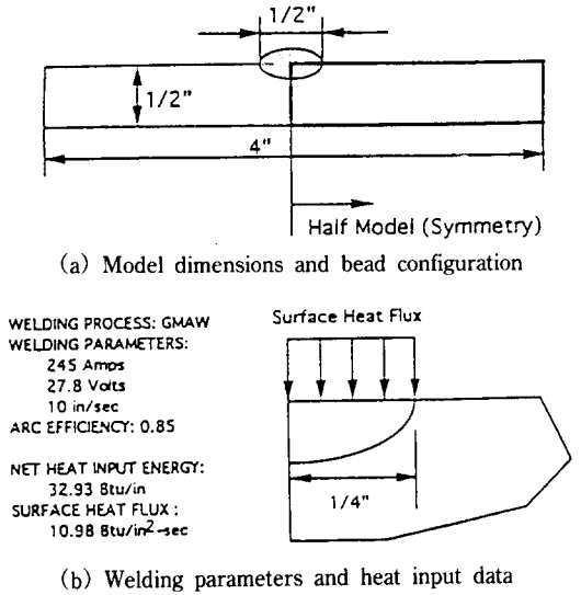
Fig. 3 Single pass bead-on-plate weld on the 1/2" thick plate
