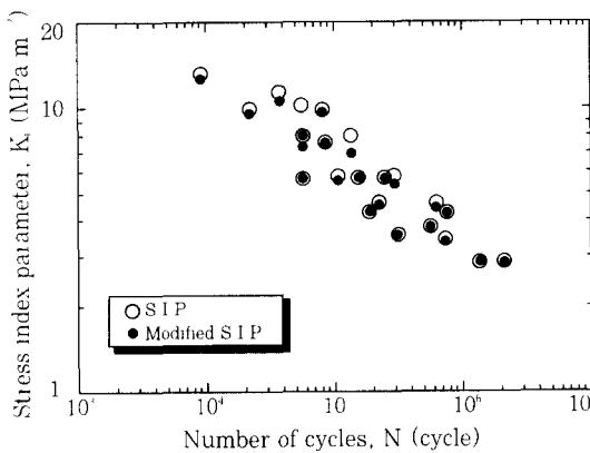
Fig. 11 Comparison of prediction methods using original and modified stress index parameter
