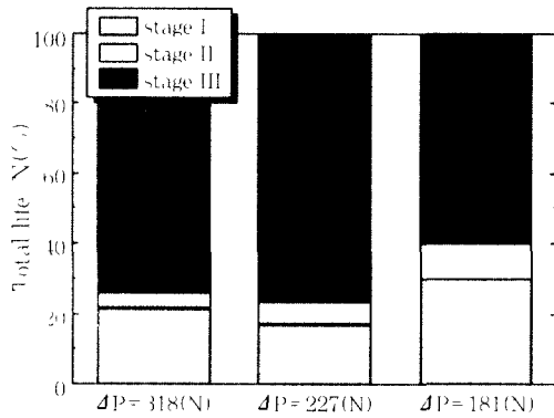
(a) L type specimen, t=1mm
