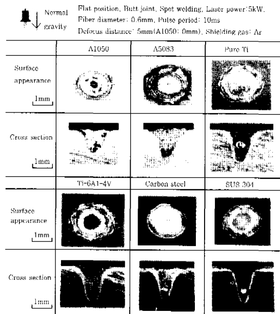
Fig. 5 Weld quality with standard rectangular pulse waveform
