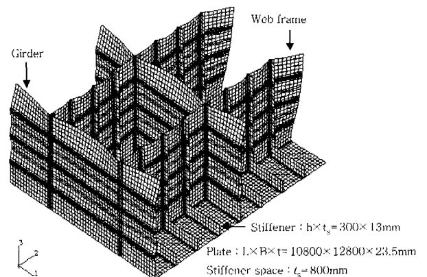
Fig. 8 Simulation result for tank top block model with carlings at sub-assembly stage
