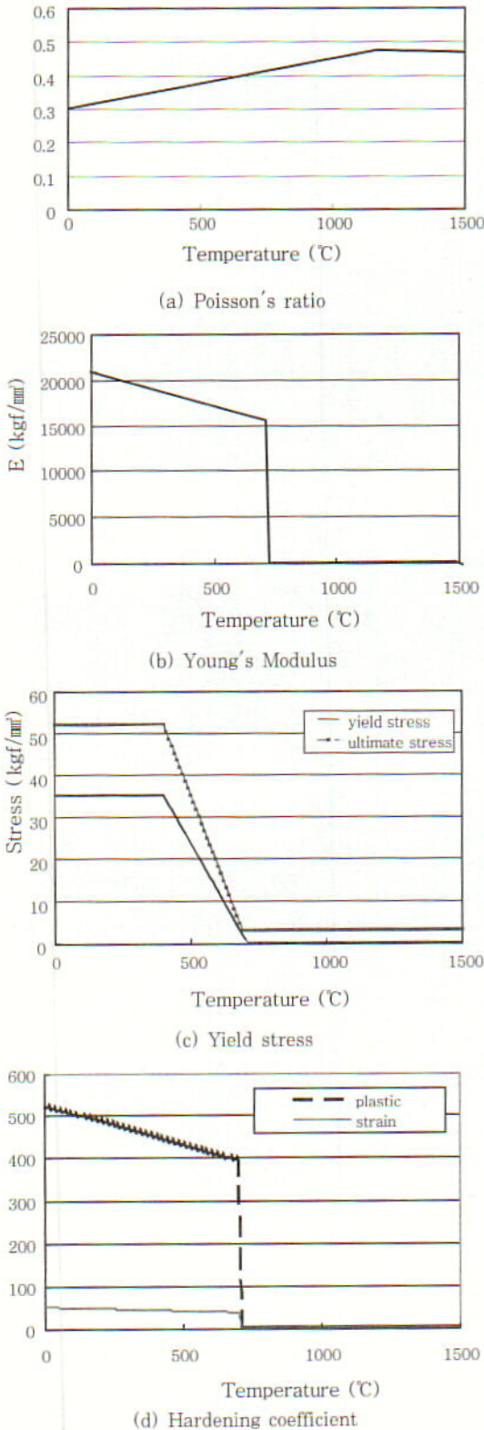
Fig. 3 Mechanical properties of thermal dependence
