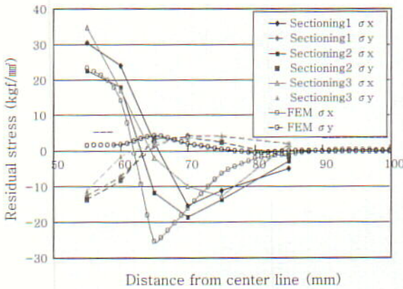
Fig. 7 Comparison FEM analysis with experiments
