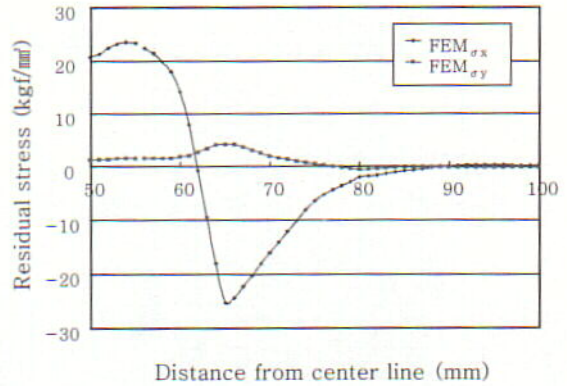
Fig. 8 FEM analysis results
