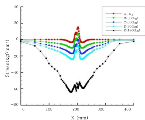
b) Stress distribution with welding residual stress
