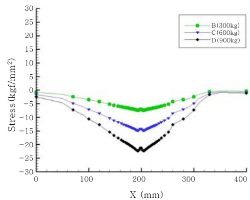
a) Stress distribution without welding residual stress
