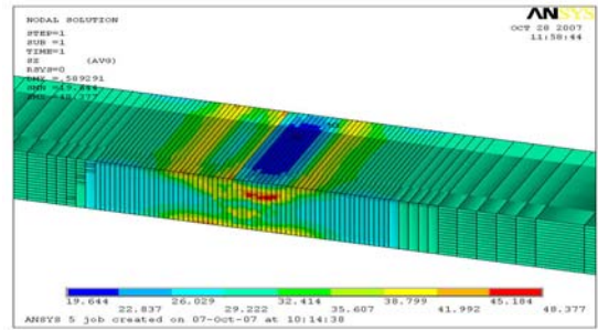
a) Stress distribution under tensile load
