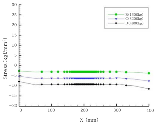
a) Stress distribution without welding residual stress
