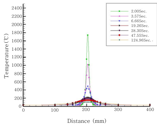
Fig. 3 Temperature history(W.M,H.A.Z,B.M.)
