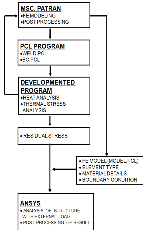
Fig. 1 Schematic diagram for externally loaded welded structure analysis
