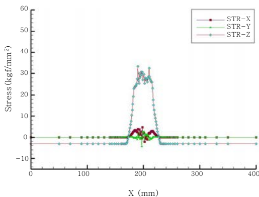
Fig. 5 Distribution of welding residual stress in the weld joint
