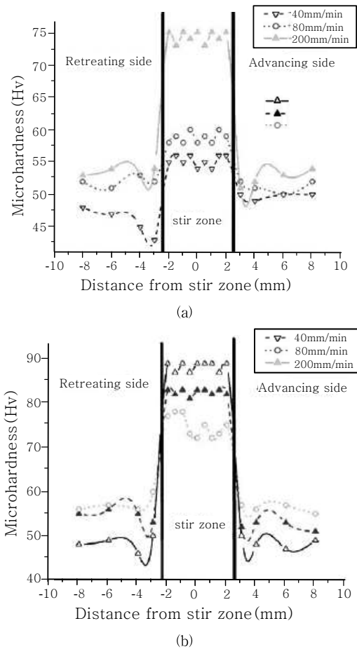
Fig. 7 Microhardness values of specimens FSPed (a) without SiC particles and (b) with SiC particles in different traverse speeds 16)
