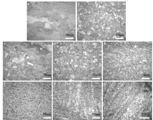
Fig. 5 OM micrographs of (a) base metal, stir zone of specimens FSPed without SiC particles at (b) rotational and traverse speed of 1120 rpm and 80mm/min, (c-e) rotational speed of 900 rpm and traverse speeds of 40, 80 and 200mm/min respectively, and (f-h) specimens FSPed with SiC particles at rotational speed of 900 rpm and traverse speeds of 40, 80 and 200mm/min respectively 16)
