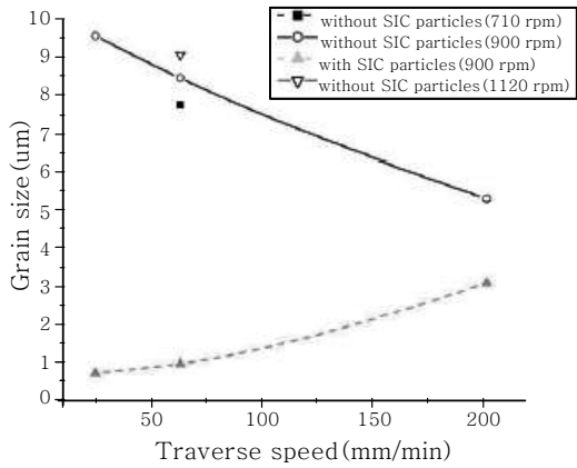
Fig. 6 Variation of grain size of specimens produced with and without SiC particles in different rotational and traverse speeds 16)
