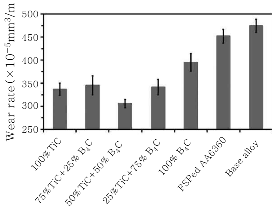
Fig. 8 Wear rate of fabricated mono and hybrid MMC 17)
