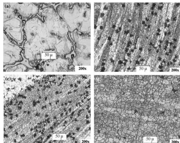
Fig. 9 Effect of alumina particle size and tool geometry on grain size and cluster size (a) base metal, (b, c, and d) FSPed specimen with 0.03, 0.3, 3 \mu\text{m} alumina particle size, respectively 18)
