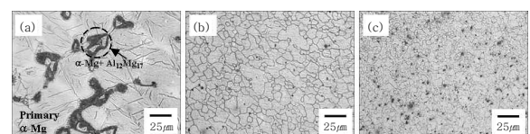
Fig. 3 Optical microstructure of AM60 : (a) base metal, (b) SZ without SiCp, (c) SZ with SiCp
