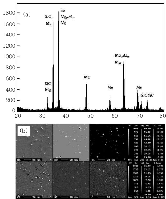
Fig. 4 Phase and chemical composition analysis of SZ with SiCp: (a) XRD analysis, (b) EPMA analysis
